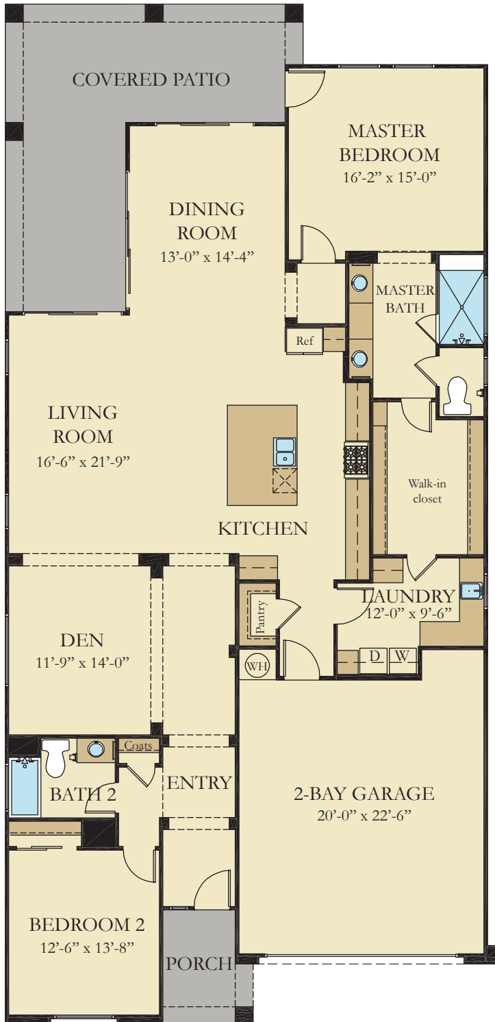
FIRST FLOOR
